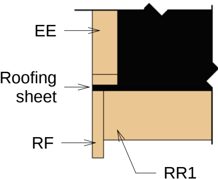
3 Roof Reinforcement
